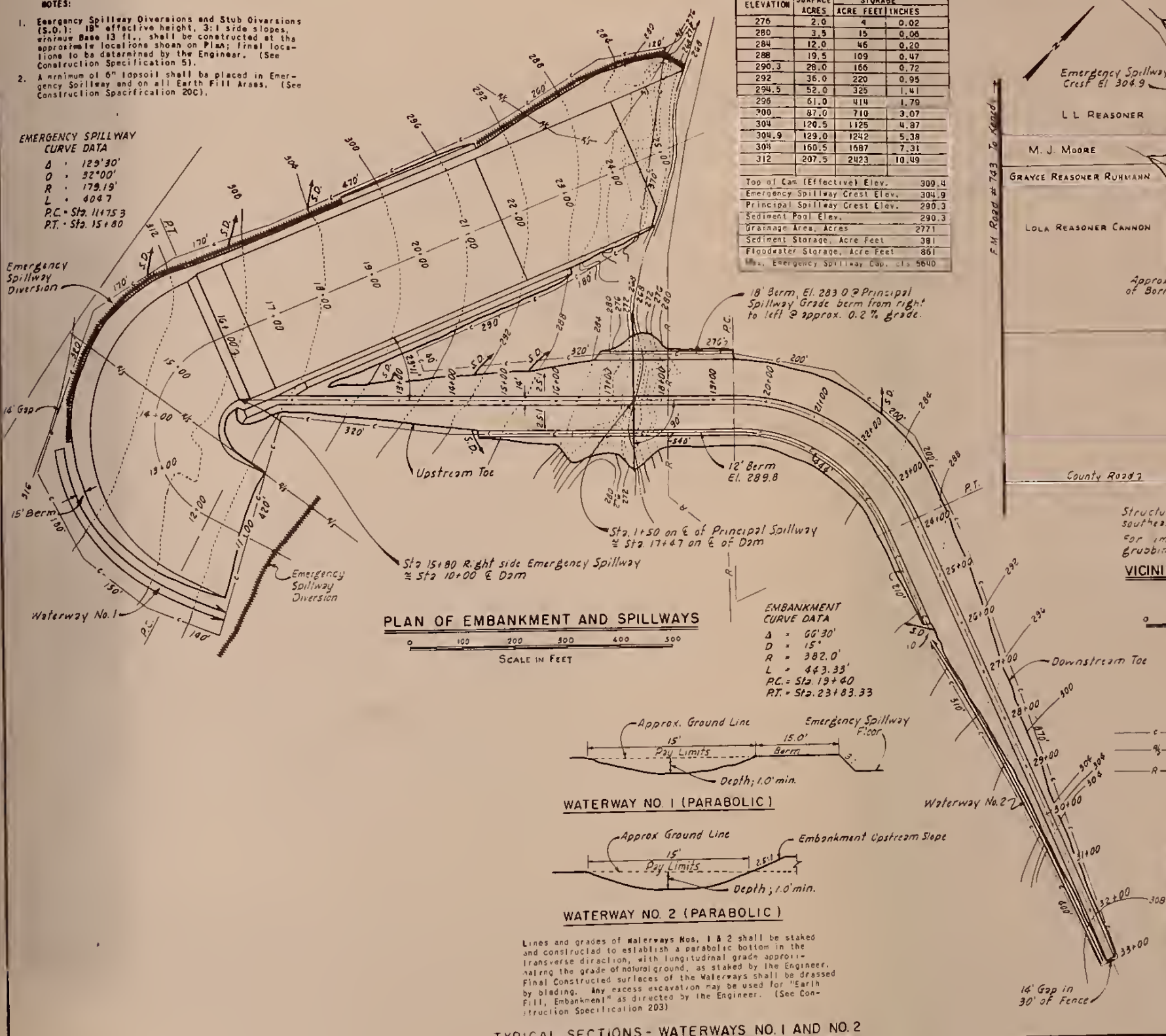
TYPICAL SECTIONS - WATERWAYS NO. 1 AND NO. 2
